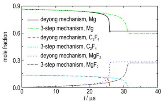
图7 Deyong机理与三步机理主要组分摩尔分数比较 Fig.7 Comparison of mole fraction for major species between Deyong and 3-step mechanisms
